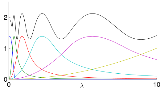
Fig. 1. Scaling function h(\lambda) (blue curve), wavelet generating kernels g(t_j\lambda) , and sum of squares G (black curve), for J = 5 scales, \lambda_{max} = 10 , K = 20 . Details in Section 8.1. (For interpretation of colors in this figure, the reader is referred to the web version of this article.)
